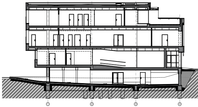
Rez
